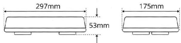
MPL300 dimensions in mm.
